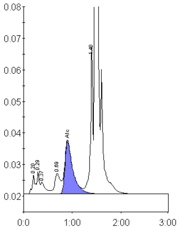
Peak table - ID: 10575829
